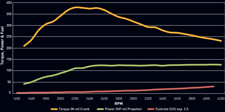
OXE 125 HP TORQUE / POWER / FUEL CONSUMPTION
