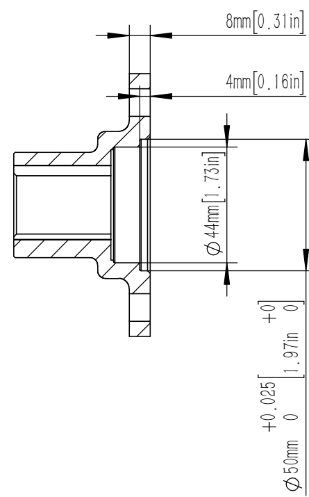
DETAIL OF FLYWHEEL SCALE 1:2
